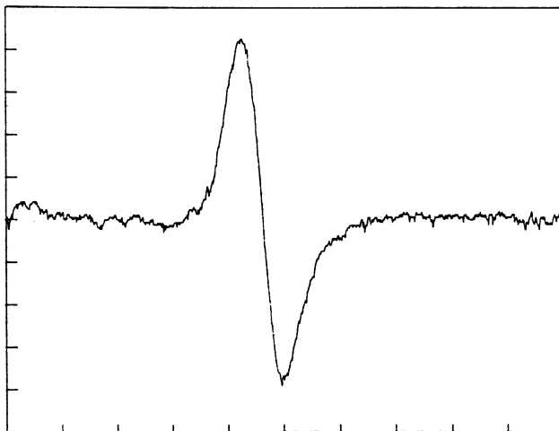
FIG. 1. Observed spectral line of the 3\nu_2 ( l = 1 ) \leftarrow 0 overtone band of \text{H}_3^+ corresponding to the J' = 1 , G' = 2 \leftarrow J = 2 , K = 2 transition at 6877.512 \text{ cm}^{-1} . Wavenumber scan is about 0.95 \text{ cm}^{-1} for the full trace. The time constant of detection is 3 sec.
